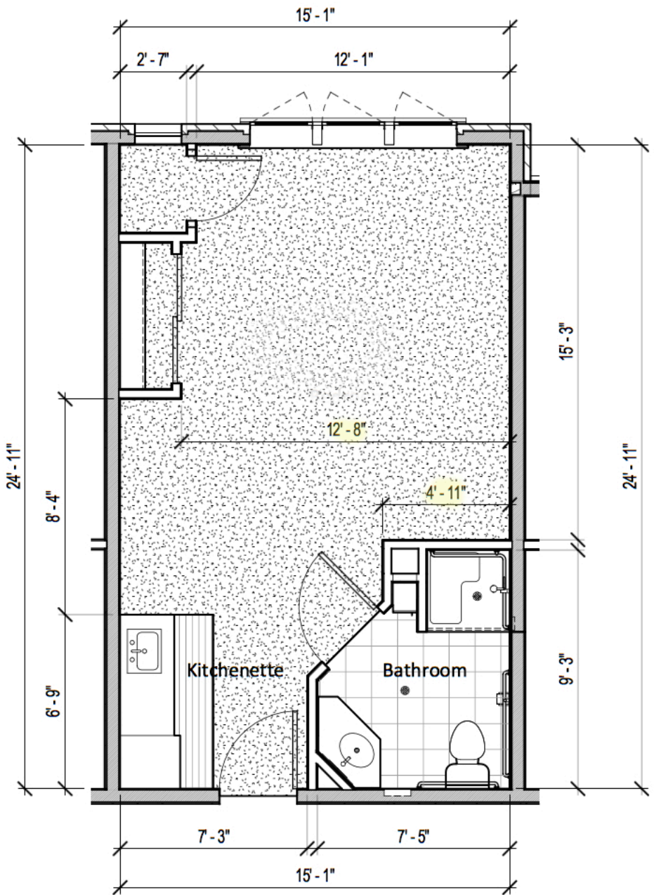
Assisted Living Studio-A (285 SF)
